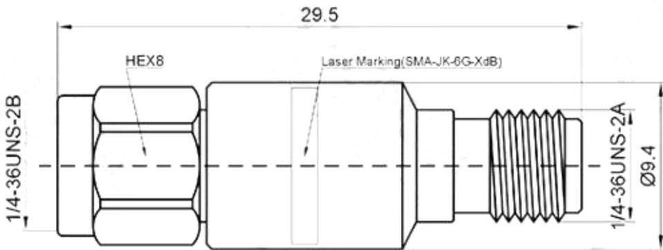
SMA Male To Female 2W 6G 20dB Fixed Attenuator
